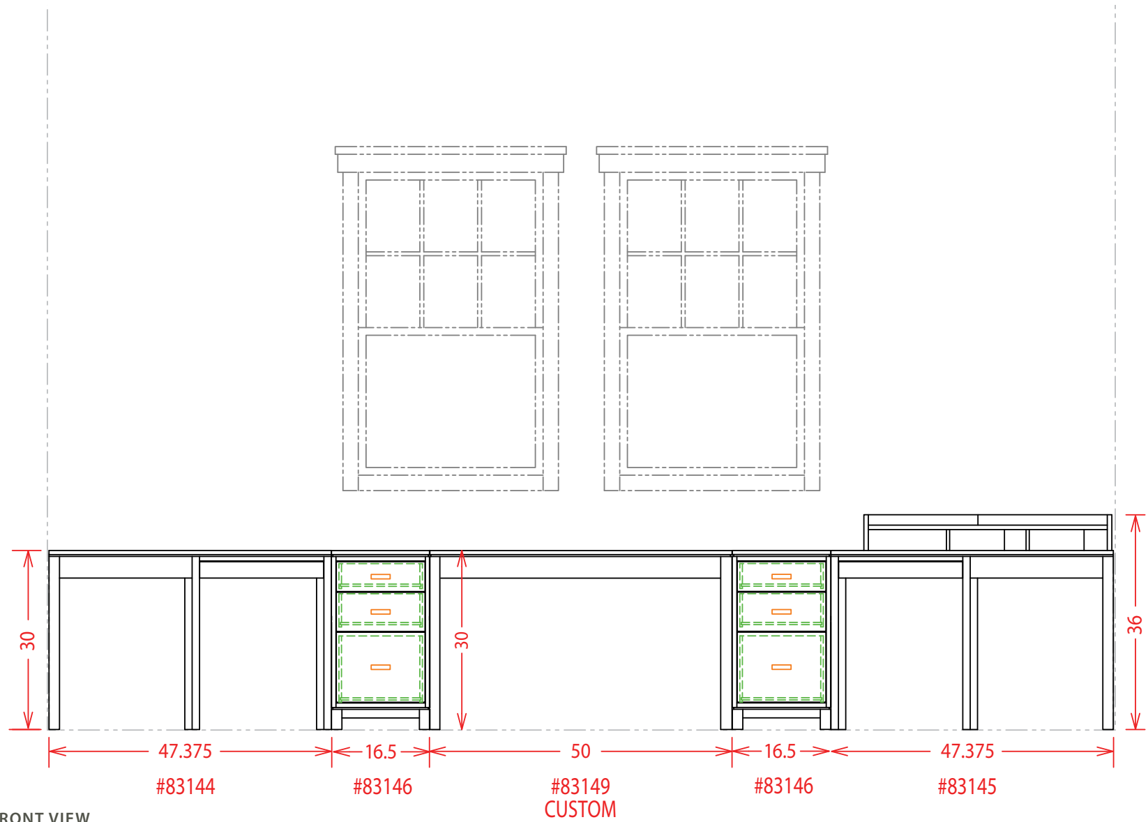
FRONT VIEW
