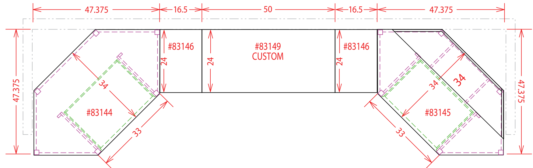
TOP VIEW
